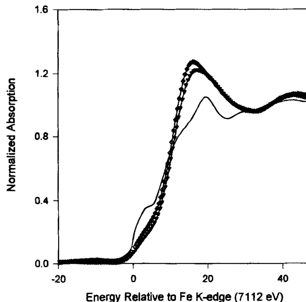
Fig. 18. Fe K-edge XANES for the PtFe/C electrocatalyst at 0.54 V ( \nabla ) and 0.84 V ( \diamond ) relative to an Fe foil standard (—).
