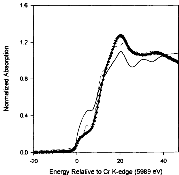
Fig. 16. Cr K-edge XANES for the PtCr/C electrocatalyst at 0.54 V ( \nabla ) and 0.84 V ( \diamond ) relative to Cr 2 O 3 (---) and Cr foil standard (—).
