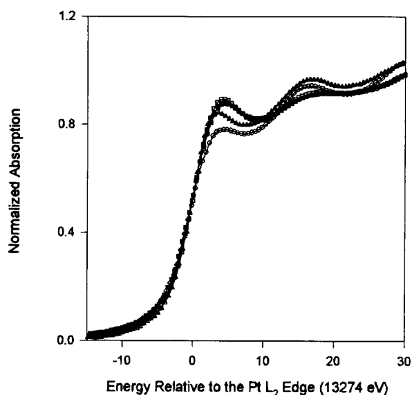
Fig. 6. XANES spectra at the Pt L 2 edge for (a) PtCr/C (●), PtMn/C (▽), PtFe/C (▼) and (b) Pt/C (△), PtCo/C (□), PtNi/C (■) relative to a Pt reference foil (○) at 0.54 V in 1M HClO 4 .
