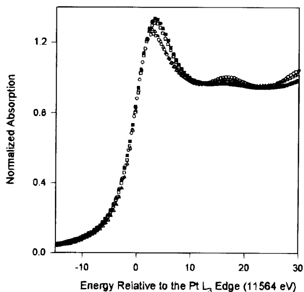
Fig. 5. XANES spectra at the Pt L 3 edge for (a) PtCr/C (●), PtMn/C (▽), PtFe/C (▼) and (b) Pt/C (△), PtCo/C (□), PtNi/C (■) relative to a Pt reference foil (○) at 0.54 V in 1M HClO 4 .
