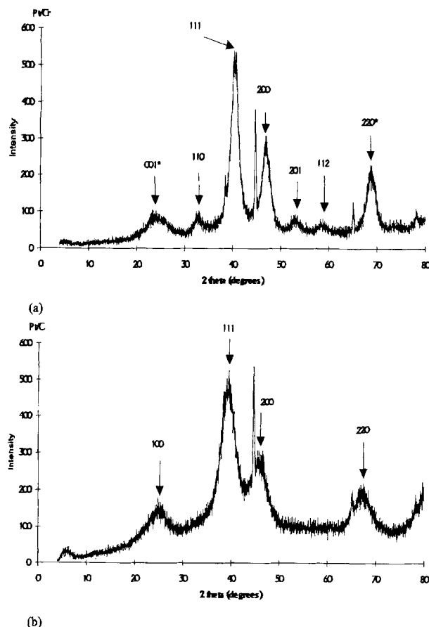
Fig. 3. XRD pattern for (a) PtCr/C electrocatalyst. Primary phase is Li 2 type with fcc lattice. Contribution from secondary phase {*} (Li 6 type with tetragonal lattice structure) is ~9% and (b) Pt/C electrocatalyst.
