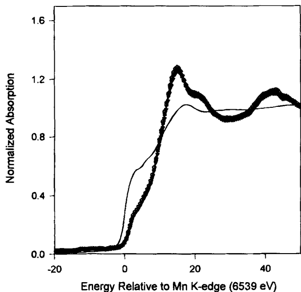
Fig. 17. Mn K-edge XANES for the PtMn/C electrocatalyst at 0.54 V ( \nabla ) and 0.84 V ( \diamond ) relative to an Mn foil standard (—).
