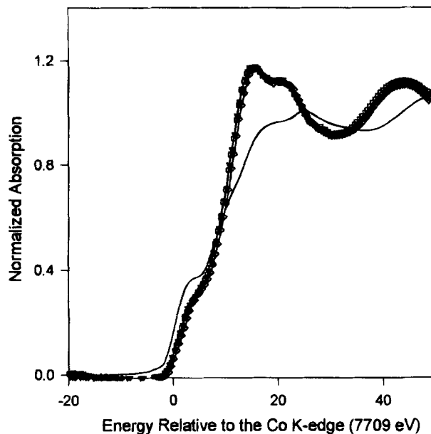
Fig. 19. Co K-edge XANES for the PtCo/C electrocatalyst at 0.54 V ( \nabla ), 0.84 V ( \diamond ), and 1.14 V ( \square ) relative to a Co foil standard (—).
