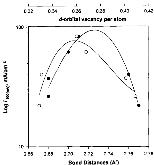
Fig. 14. Correlation of oxygen electrode performance ( \text{Log } i_{900\text{mV}} , \text{mA cm}^{-2} ) of Pt and Pt alloy electrocatalysts in PEMFC with Pt-Pt bond distance (●) and the d -orbital vacancy of Pt (○) obtained from in situ XAS.
