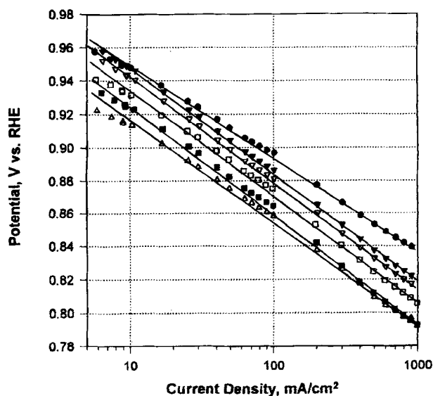
Fig. 2. iR -corrected Tafel plots for oxygen reduction in PEMFCs at 95^\circ\text{C} and 5 atm pressure for Pt and Pt alloy electrocatalysts, Pt loading on electrodes 0.3 \text{ mg cm}^{-2} . PtCr/C (●); PtMn/C (▽); PtFe/C (▼); PtCo/Co (□); PtNi/C (■); and Pt/C (△).
