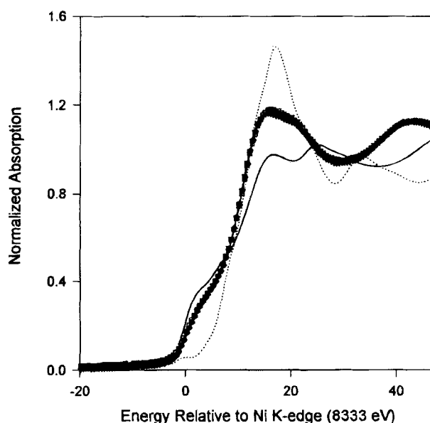
Fig. 15. Ni K-edge XANES for the PtNi/C electrocatalyst at 0.54 V (▽), 0.84 V (◇), and 1.14 V (□) relative to NiO (---) and Ni foil standard (—).
